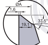
BEVEL FOR WALL THICKNESS W.T GREATER THAN 22.35mm DETAIL OF "C" (26"~48")
