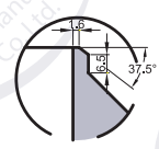
BEVEL FOR WALL THICKNESS W.T FROM 5mm TO 22.35mm INCLUSIVE DETAIL OF "C" (1/2"~24")
