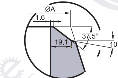
BEVEL FOR WALL THICKNESS W.T. GREATER THAN 22.35mm DETAIL OF "C" (26"~36")
