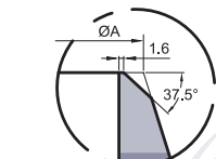
BEVEL FOR WALL THICKNESS W.T FROM 5mm TO 22.35mm INCLUSIVE DETAIL OF "A"
