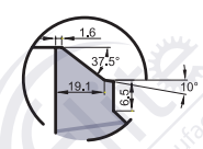
BEVEL FOR WALL THICKNESS W.T GREATER THAN 22.35mm DETAIL OF "C" (1/2"~24")
