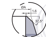
BEVEL FOR WALL THICKNESS W.T. FROM 5mm TO 22.35mm INCLUSIVE
